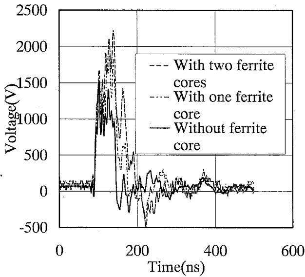
(a) Voltage wave form
