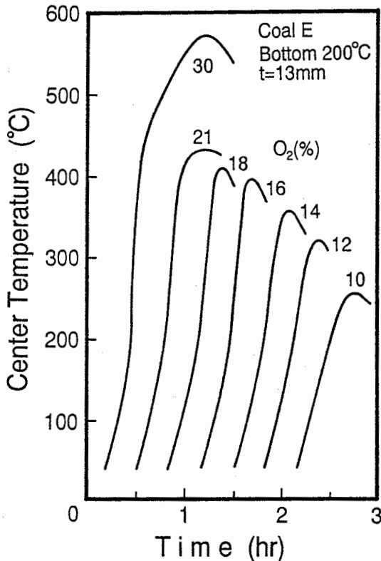
Fig. 11 Effect of O 2 concentration on the center temperature in N 2 -O 2 atmospheres for coal E 昇温曲線への酸素濃度の影響 (N 2 -O 2 系)
