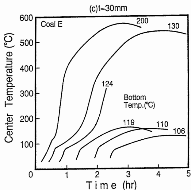
Fig. 7 Effects of thickness and bottom temperature on time history of the center temperature for coal E 昇温曲線に対する堆積厚と下面温度の影響
