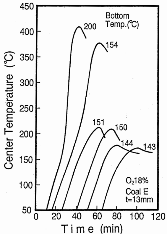
Fig. 10 Variation of the center temperatures with time using N 2 as the diluent for coal E 窒素添加雰囲気での試料 E の昇温曲線
