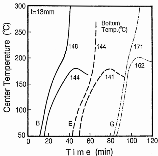
Fig. 8 Variation of the center temperature with time at around the critical ignition temperatures for coal B, E and G 試料 B, E, G の自然発火限界温度付近での昇温曲線
