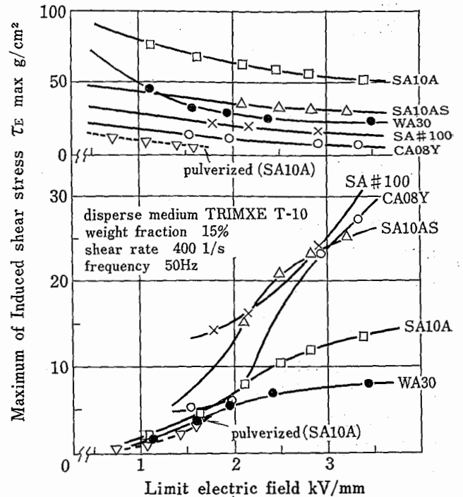
Fig.7 Characteristic scheme of maximum induced shear stress in case of anion exchange resins
