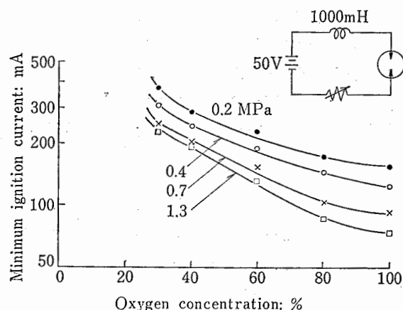
Fig. 5 Influence of oxygen and total pressure on minimum ignition current for Japanese paper by inductive sparks in O 2 /He atmospheres.
