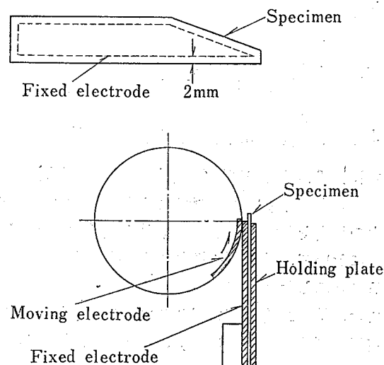
Fig. 1 Attachment of test specimen to fixed electrode of break-flash apparatus.
