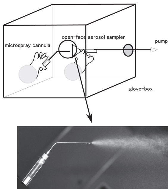
Fig. 1. The experimental set-up was installed in a glove-box (A). Aerosolized MWCNT suspension was ejected into the air from the tip of a microspray cannula which was connected with a syringe filled with the MWCNT suspension (B). The concentration of MWCNT suspension used was 533 \mu\text{g/ml} (equivalent to a dose of 160 \mu\text{g} in 0.3 \text{ ml} suspension).
